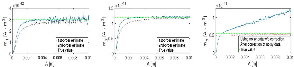
Figure 2. Estimates for m_1 (left), m_2 (center), m_3 (right) versus A , with noise of SNR=20.
